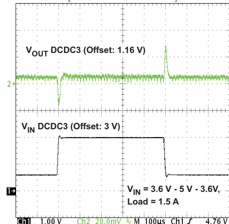
Figure 17. Line Transient Response Converter 3
