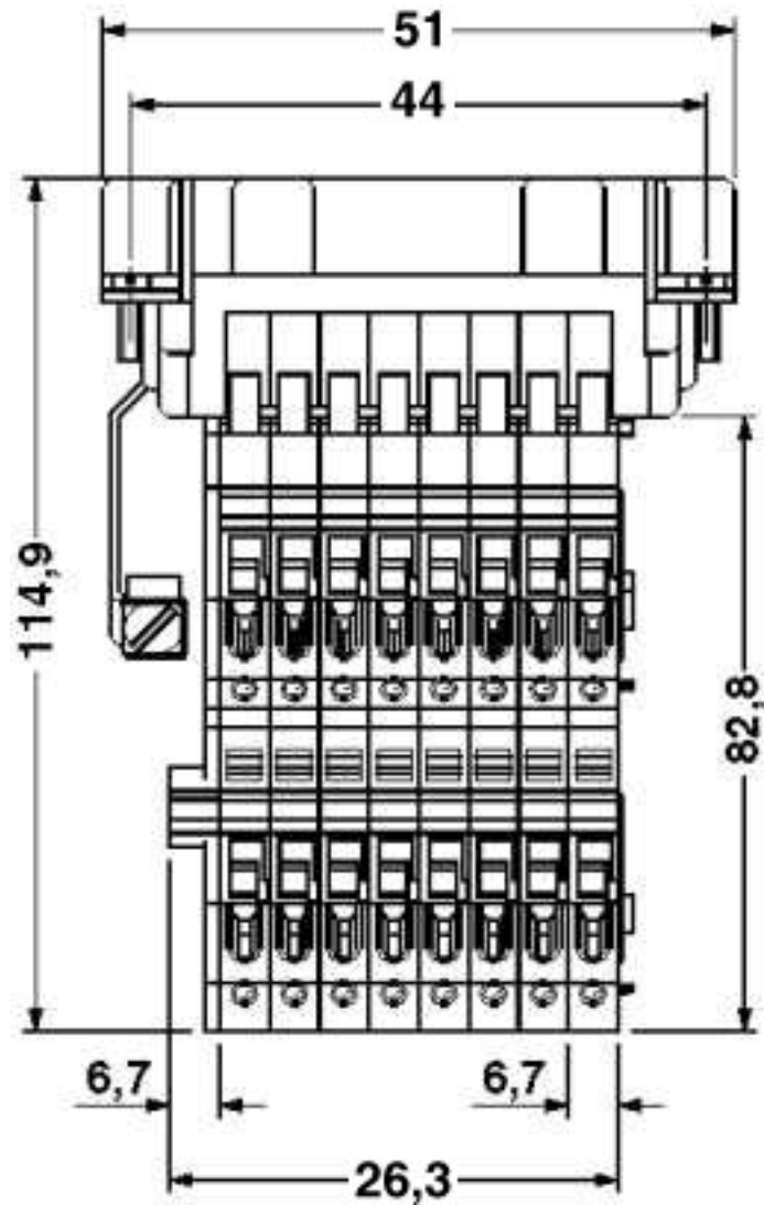
Dimensioned drawing
