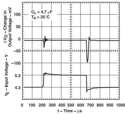
Figure 7-4. TPS76633 Line Transient Response (Legacy Chip)
