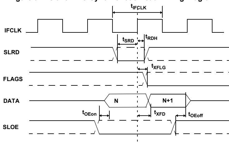
Figure 9-7. Slave FIFO Synchronous Read Timing Diagram [20]
