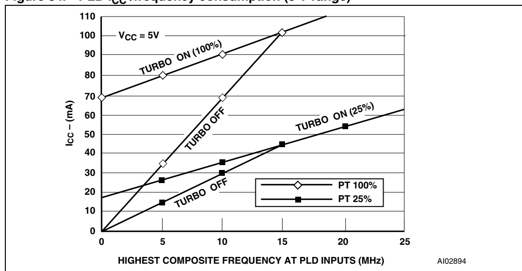
Figure 84. PLD I_{CC} /frequency consumption (5 V range)
