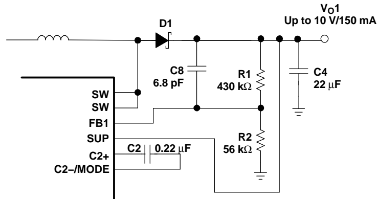
Figure 15. Feedforward Capacitor
