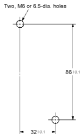
Mounting Hole Dimensions (TOP VIEW)
