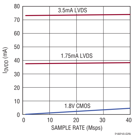
LTC2181: I_{OVPD} vs Sample Rate, 5MHz, -1dBFS, Sine Wave Input on Each Channel
