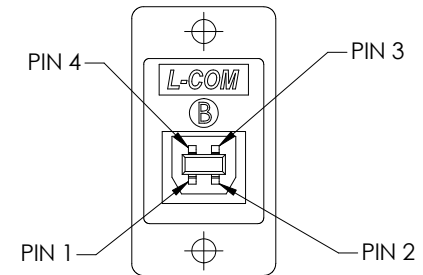
TYPE "B" JACK SHOWN
