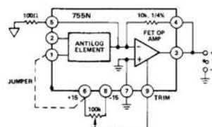
Figure 5. Trimming E_{OS} in Antilog Mode
