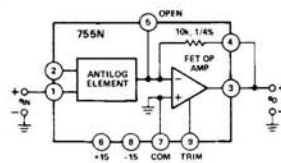
Figure 4. Functional Block Diagram
