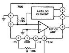
Figure 3. Trimming E_{OS} in Log Mode
