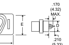
Solder Pot
