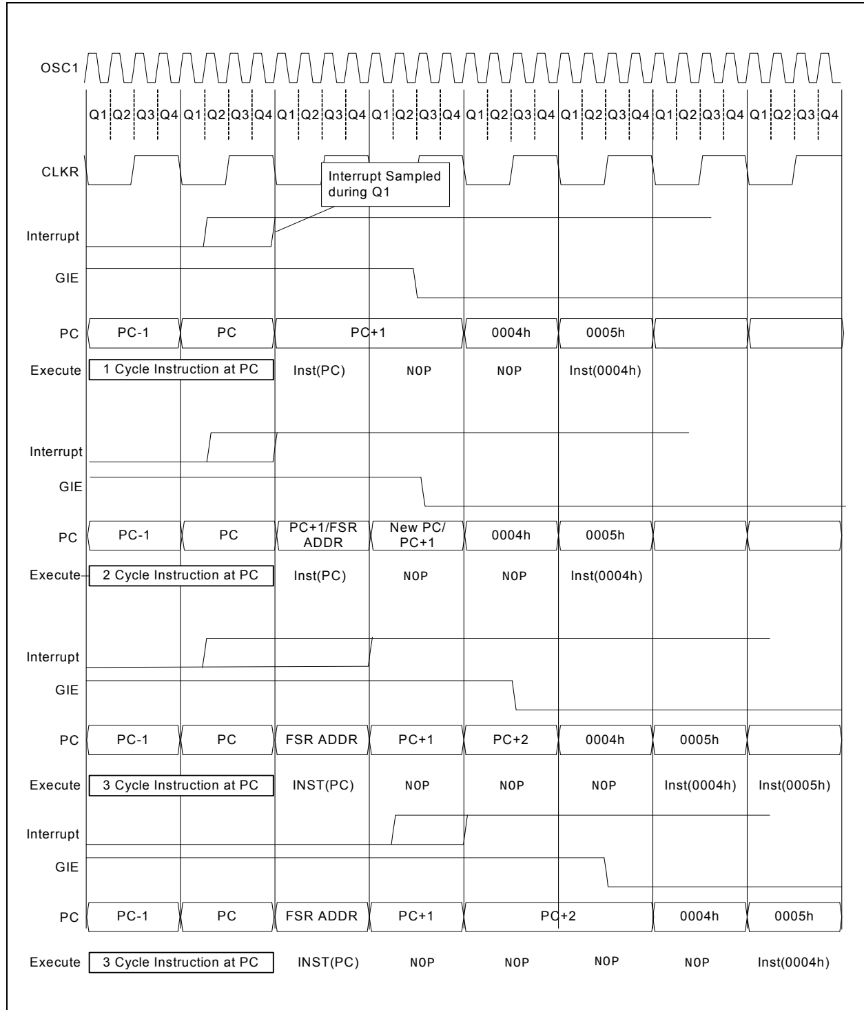
FIGURE 8-2: INTERRUPT LATENCY
