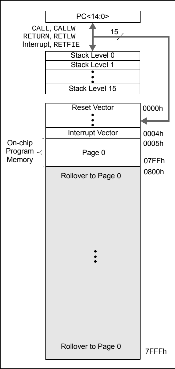
FIGURE 3-1: PROGRAM MEMORY MAP AND STACK FOR PIC16F1786
