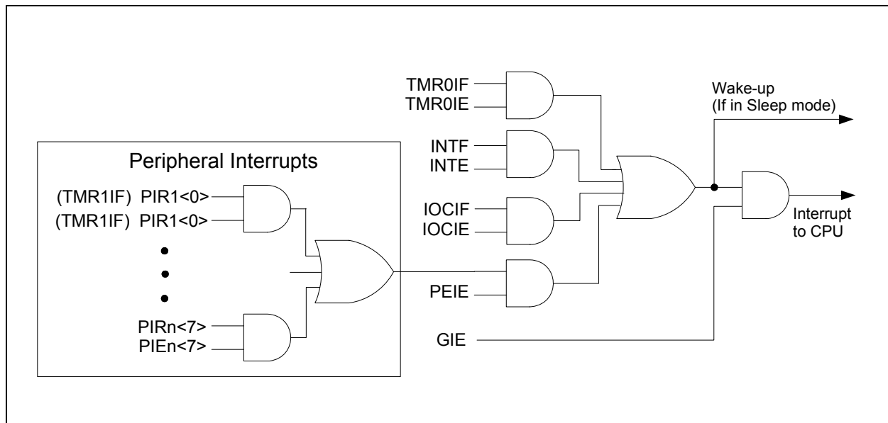
FIGURE 8-1: INTERRUPT LOGIC
