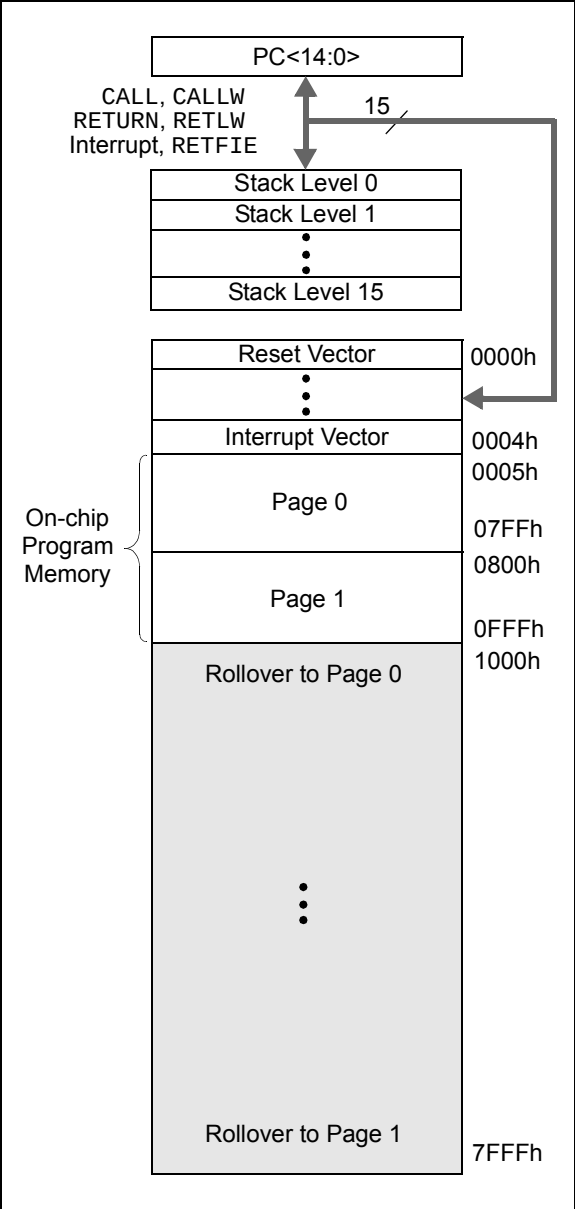
FIGURE 3-2: PROGRAM MEMORY MAP AND STACK FOR PIC16F1784/7
