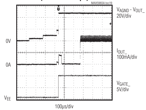
STARTUP WITH VALID PD (25k \Omega AND 0.1µF)
