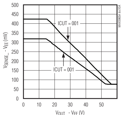
FOLDBACK CURRENT-LIMIT THRESHOLD vs. OUTPUT VOLTAGE
