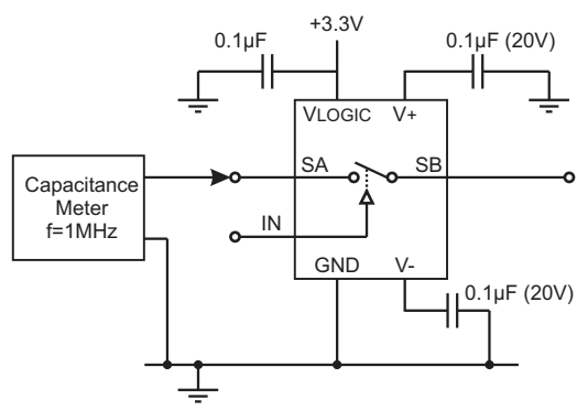
Figure 8 - Off Capacitance
