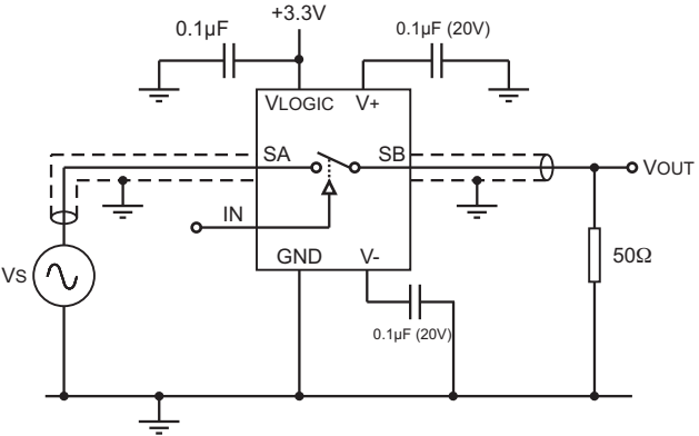
Figure 6 - Off Isolation
