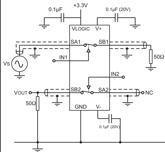
Figure 7 - Channel-to-Channel Crosstalk
