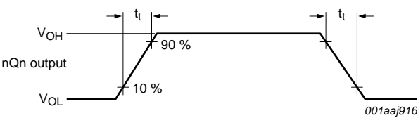
The logic levels V_{OH} and V_{OL} are typical voltage output levels that occur with the output load.
