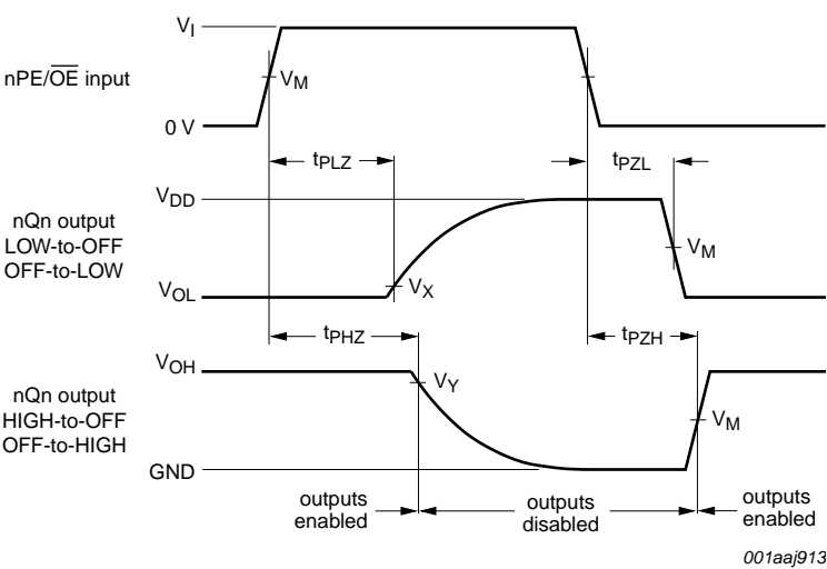
Measurement points are given in Table 9 The logic levels V_{OH} and V_{OL} are typical voltage output levels that occur with the output load.
