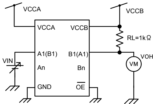
Figure 7 Test Circuit
