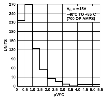
Figure 30. TCV_{OS} Distribution (J Package)
