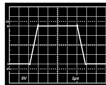
Figure 3. Excellent Output Drive, R_L = 600\text{ }\Omega
