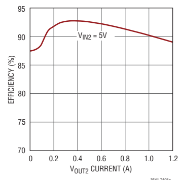
LV Channel Efficiency, 2MHz, V_{OUT2} = 3.3V
