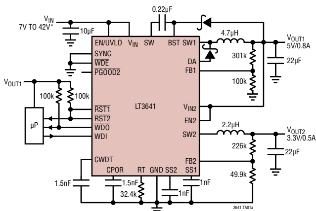
2MHz 5V/0.8A and 3.3V/0.5A Step Down Regulators
