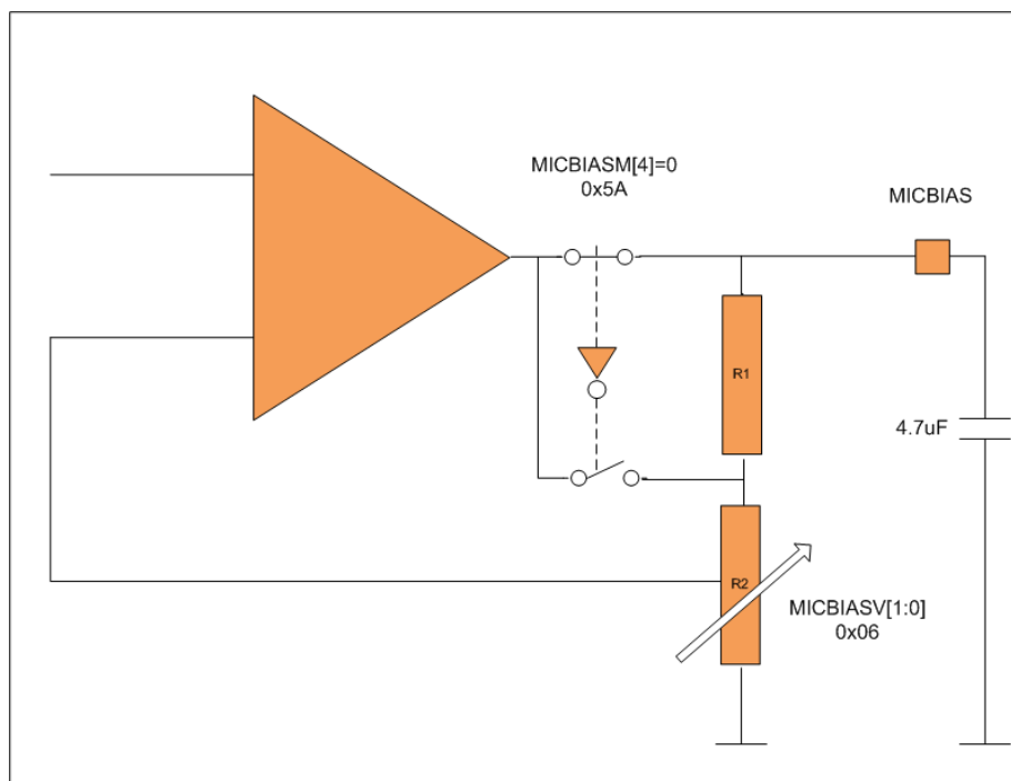
Figure 4: Microphone Bias Schematic
