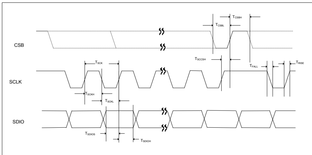
Figure 30: SPI Write Timing Diagram
