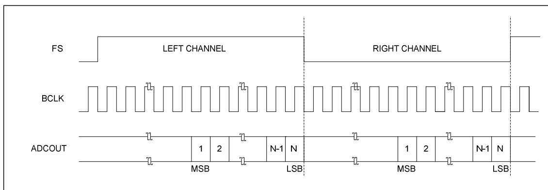
Figure 25: Right Justified Audio Interface
