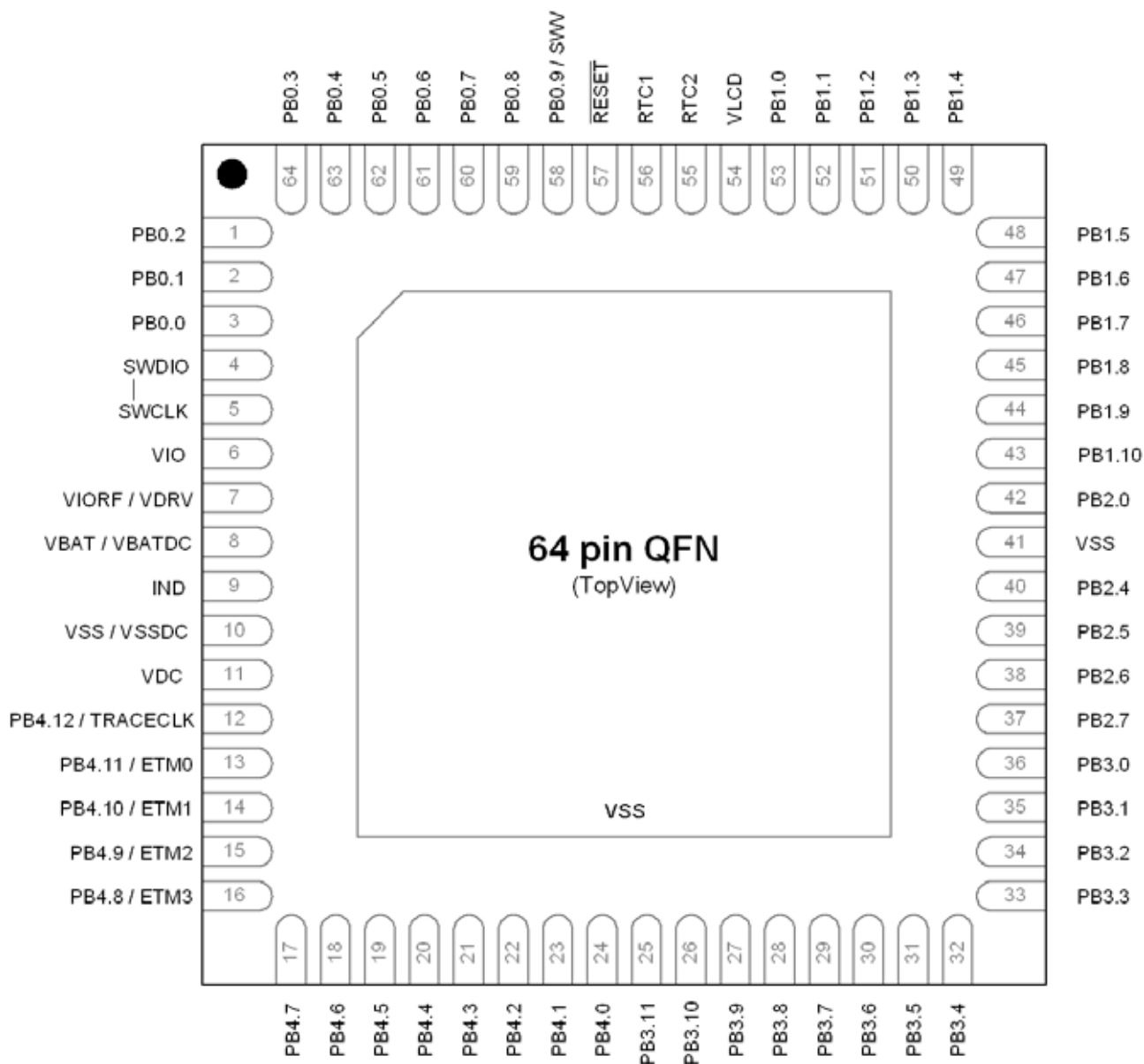
Figure 6.4. SiM3L1x6-GM Pinout
