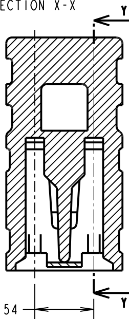
SECTION X-X
