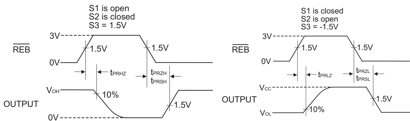
Figure 13: Receiver Enable and Disable Waveforms
