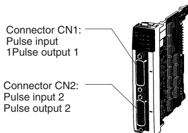
CQM1H-PLB21 Pulse I/O Board
