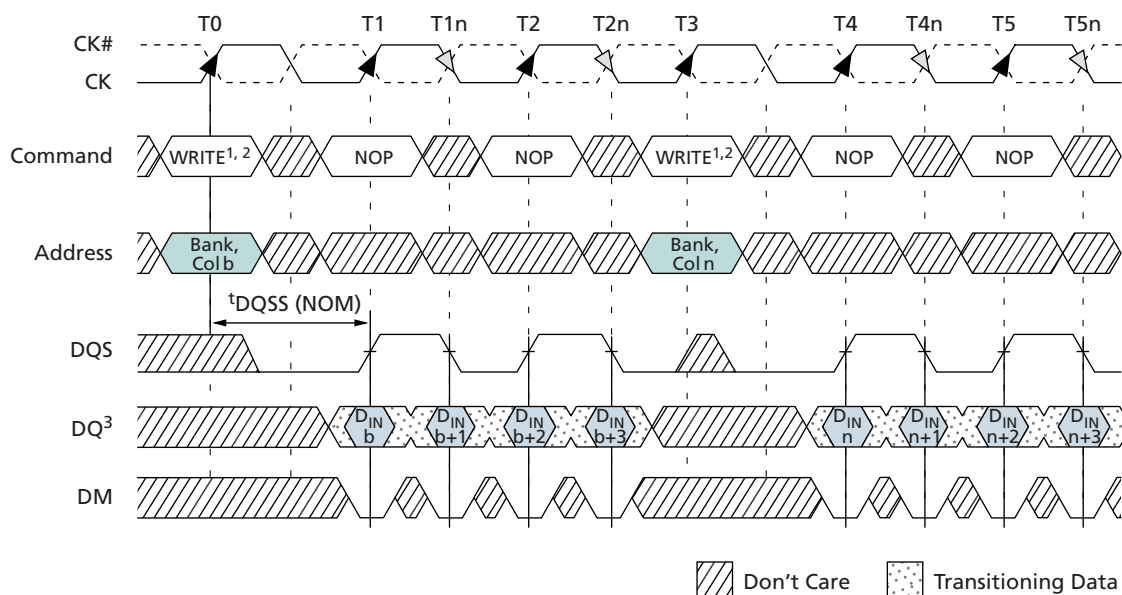
Figure 45: Nonconsecutive WRITE-to-WRITE
