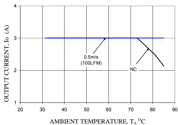
V_o = 3.3V
