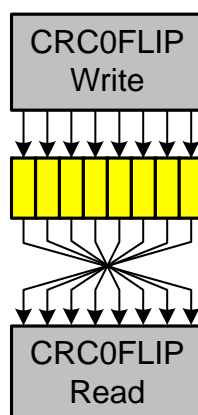
Figure 16.2. Bit Reverse Register
