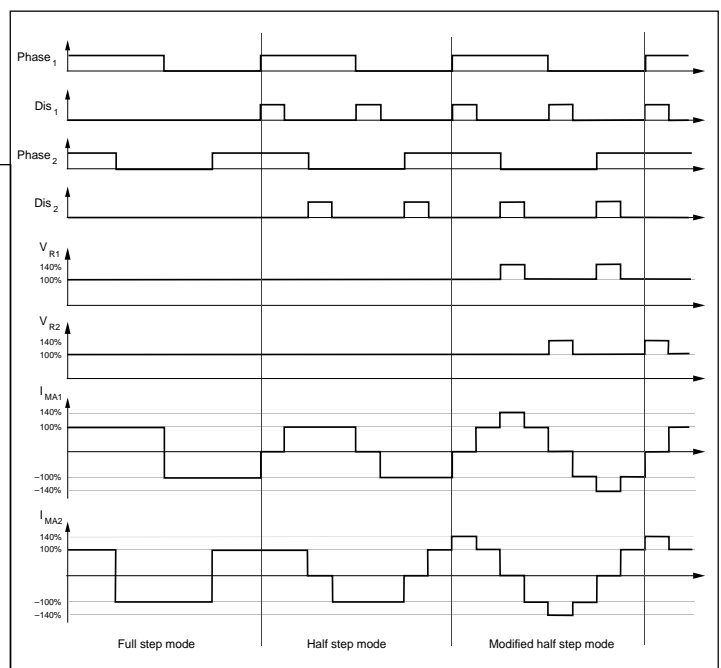
Figure 9. Stepping modes
