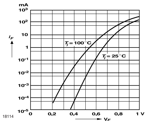
Figure 1. Forward characteristics
