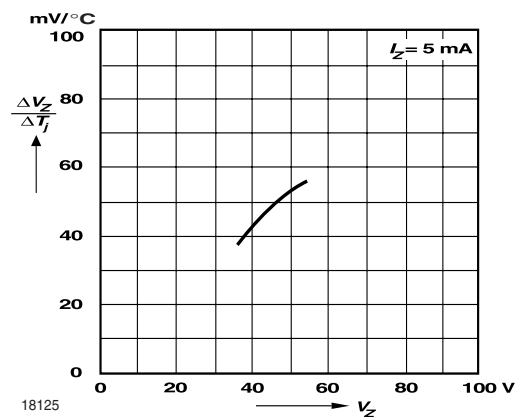
Figure 12. Temperature dependence of Zener voltage versus Zener voltage
