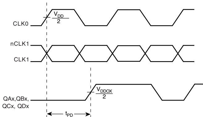
PROPAGATION DELAY
