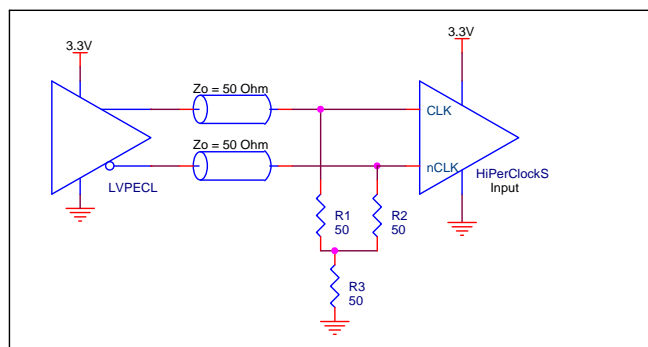
FIGURE 2B. CLK/nCLK INPUT DRIVEN BY 3.3V LVPECL DRIVER
