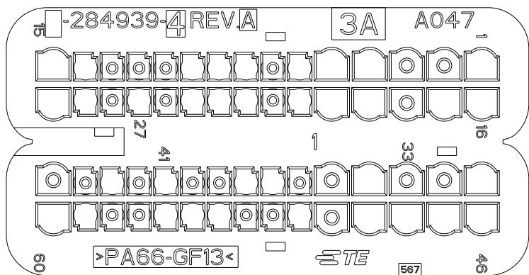
P/N 284939-4 AS SHOWN (VERDE / GREEN)
