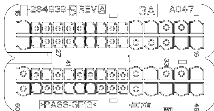
OBSOLETE P/N 284939-5 AS SHOWN (BLU / BLUE)
