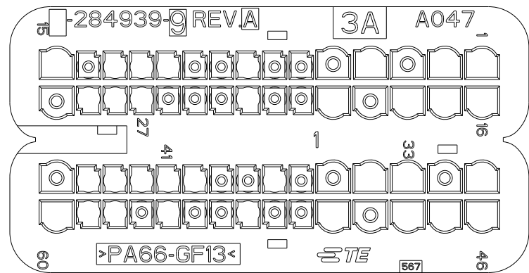
OBSOLETE P/N 284939-9 AS SHOWN (VERDE / GREEN)
