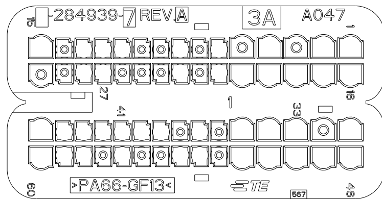
OBSOLETE P/N 284939-7 AS SHOWN (GRIGIO / GREY)
