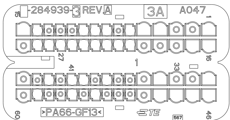
P/N 284939-3 AS SHOWN (MARRONE / BROWN)
