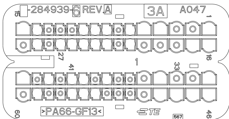
P/N 284939-6 AS SHOWN (NERO / BLACK)
