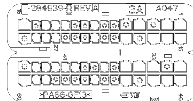
OBSOLETE P/N 284939-8 AS SHOWN (MARRONE / BROWN)
