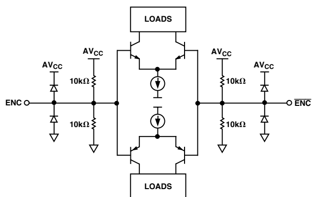
Figure 3. Encode Inputs
