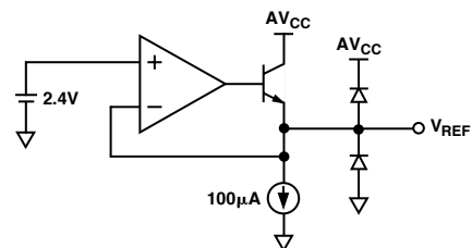
Figure 6. 2.4 V Reference
