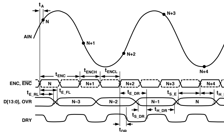
Figure 1. Timing Diagram
