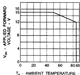
Fig. 4. Maximum Allowed Applied Forward Voltage vs. Ambient Temperature R θJA = 175°C/W 12 Volt Devices
