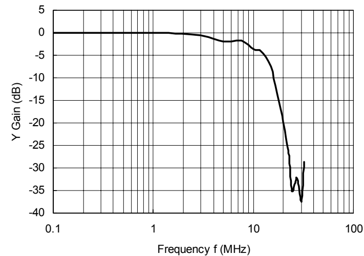
Y System Filter Characteristics (Vcc=4.8V)
