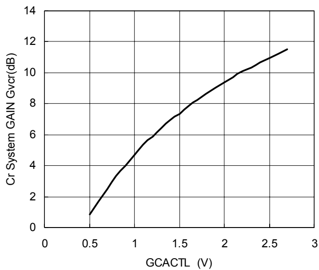
Cr System GAIN vs. GCACTL (Vcc=4.8V)
