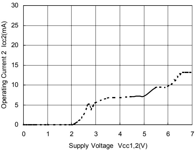
Operating Current at Power Save 2 vs. Supply Voltage (Ta=25°C)
