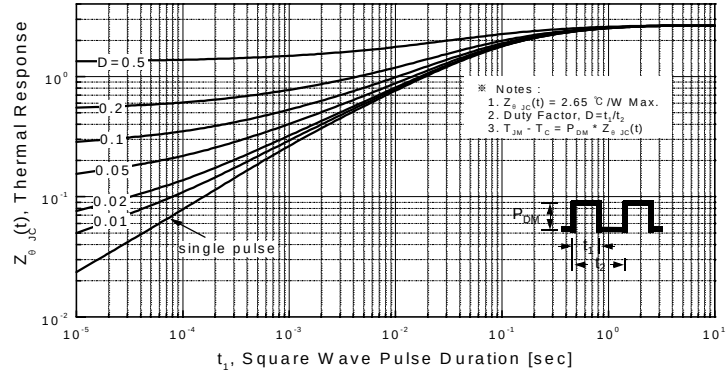
Figure 11-1. Transient Thermal Response Curve for IRF620B
