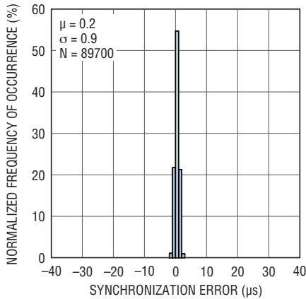
TIME n Synchronization Error 0 Packet/s Publishing Rate, 1 Hop, Room Temperature
