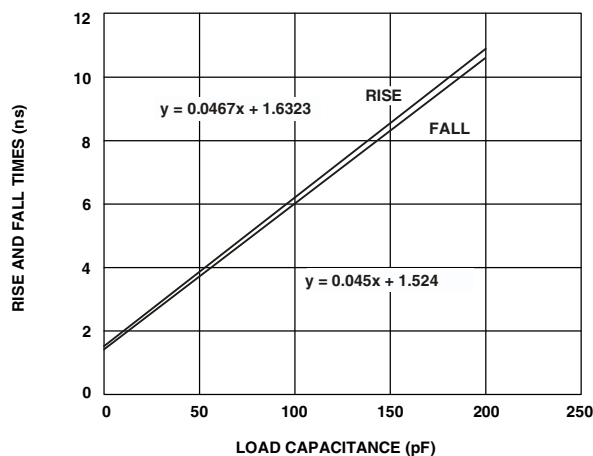
Figure 39. Typical Output Rise/Fall Time (20% to 80%, V DDEXT = Max)
