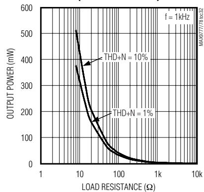
OUTPUT POWER vs. LOAD RESISTANCE (HEADPHONE MODE)
