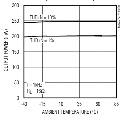
OUTPUT POWER vs. AMBIENT TEMPERATURE (HEADPHONE MODE)
