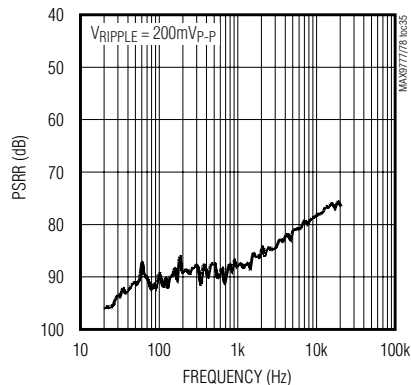
POWER-SUPPLY REJECTION RATIO vs. FREQUENCY (HEADPHONE MODE)
