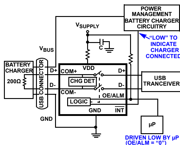
FIGURE 10. CHARGER PORT DETECTION
