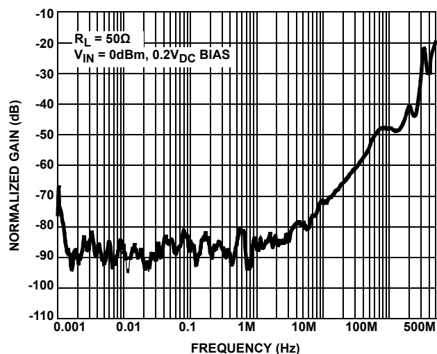
FIGURE 23. CROSSTALK
