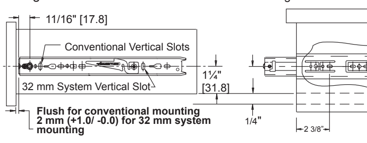
Figure 4 Conventional and 32 mm Mounting—Drawer
