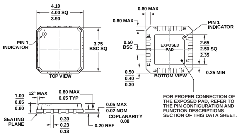
Figure 39. 20-Lead Lead Frame Chip Scale Package [LFCSP_VQ] 4 mm × 4 mm Body, Very Thin Quad (CP-20-4) Dimensions shown in millimeters
