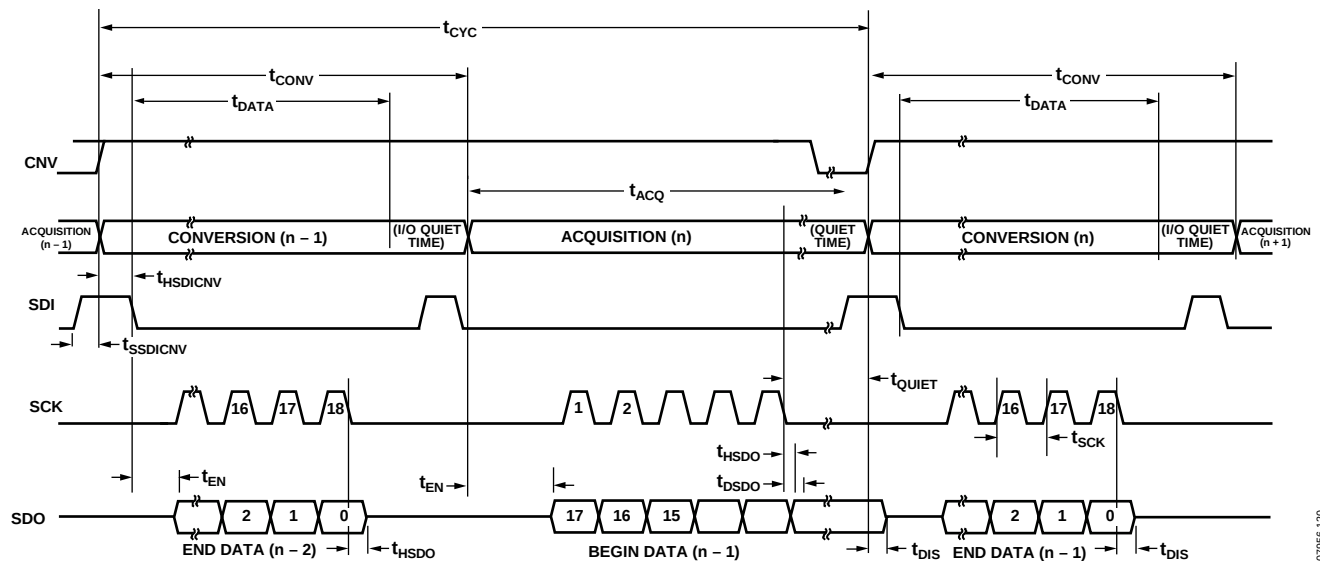
Figure 30. \overline{\text{CS}} Mode, 4-Wire Without Busy Indicator Serial Interface Timing
