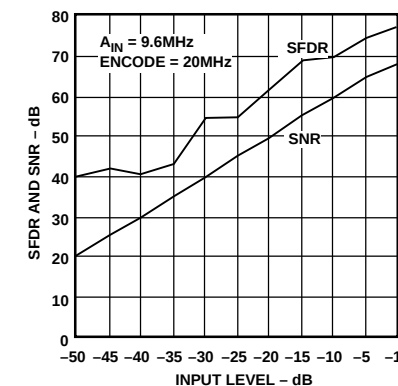
Figure 7. SFDR and SNR vs. Analog Input Level
