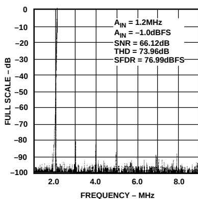
Figure 8. FFT Plot
