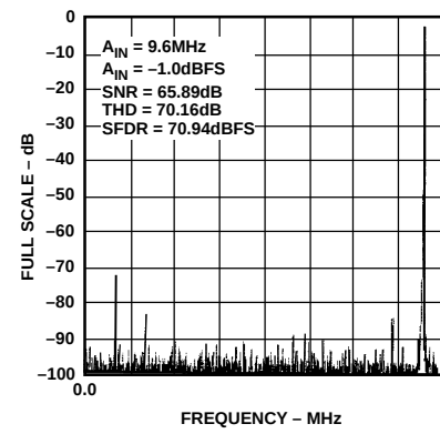
Figure 9. FFT Plot
