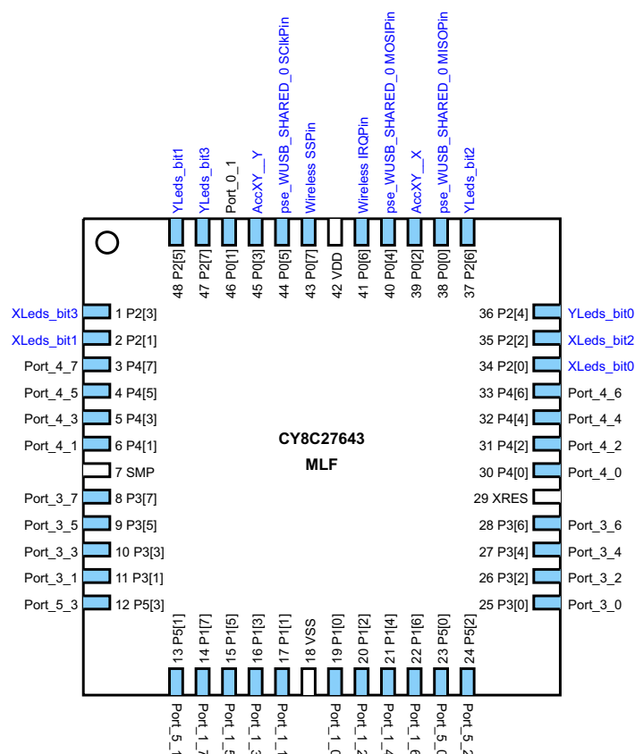
Figure 8-1. CY3209WUSBTiltSlave Pinouts
