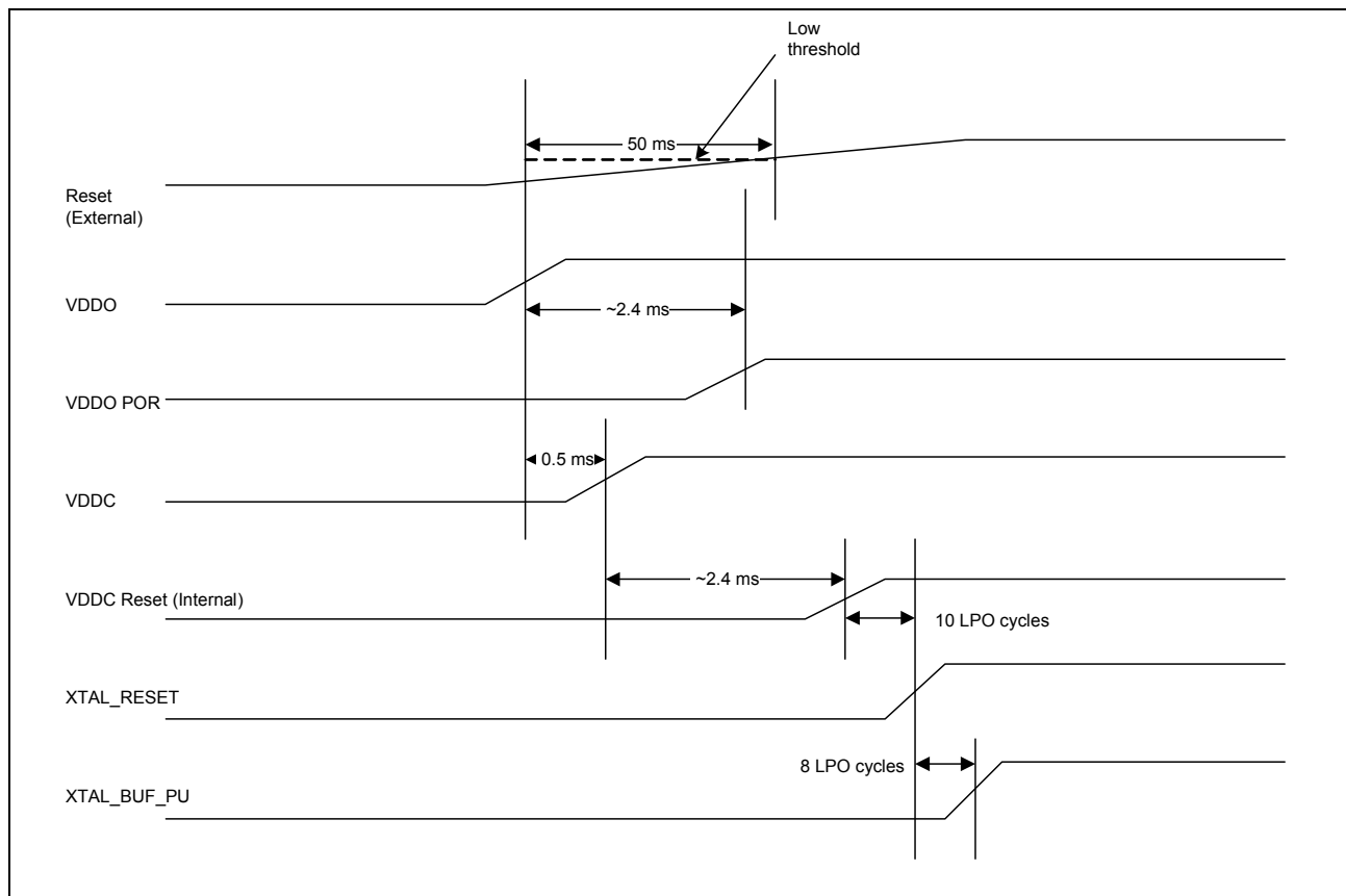
Figure 2: Reset Timing
