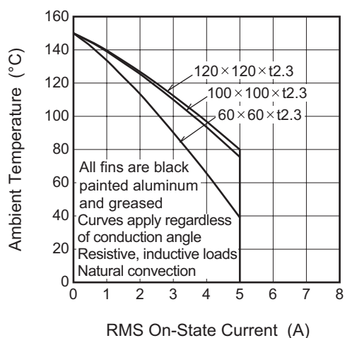
Allowable Ambient Temperature vs. RMS On-State Current
