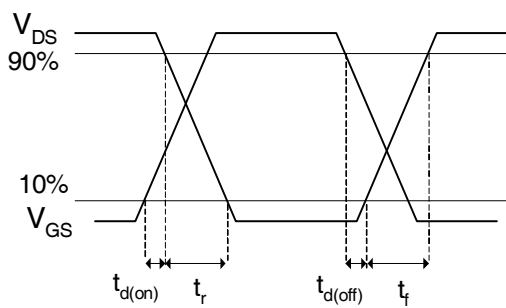
Fig 23b. Switching Time Waveforms
