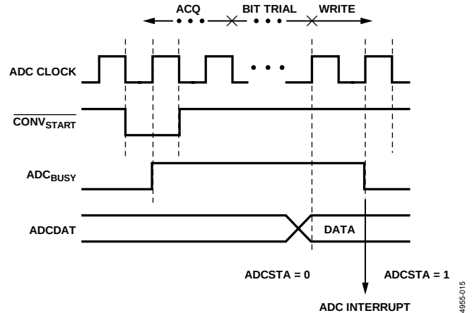
Figure 40. ADC Timing
