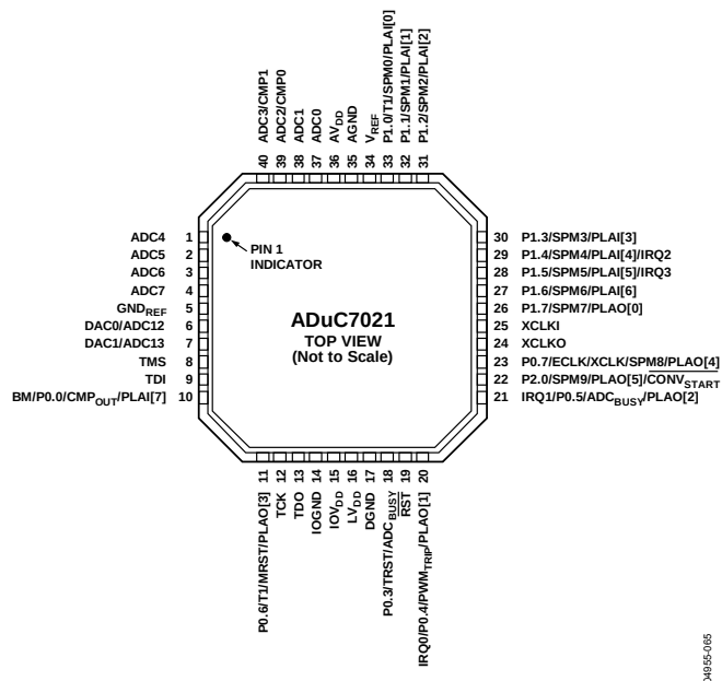
Figure 11. ADuC7021 40-Lead LFCSP_VQ Pin Configuration
