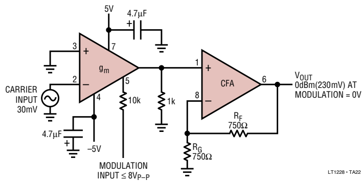
Amplitude Modulator
