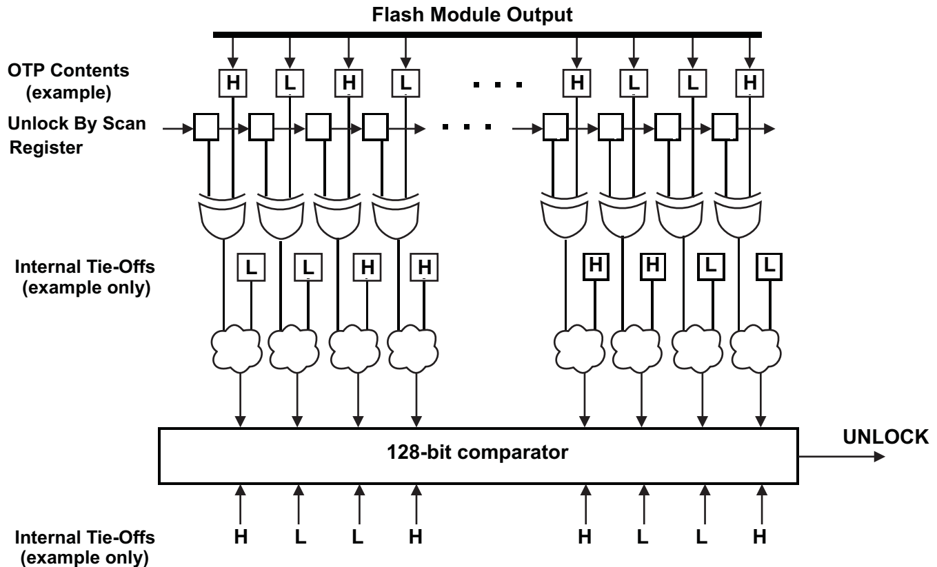
Figure 4-15. AJSM Unlock
