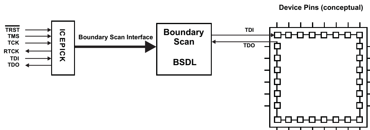
Figure 4-16. Boundary Scan Implementation (Conceptual Diagram)
