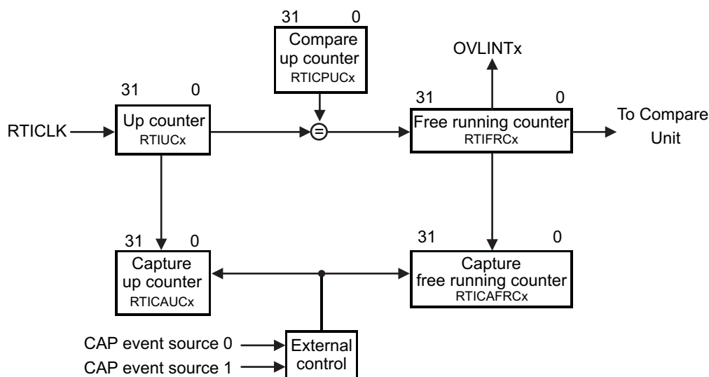
Figure 4-11. Counter Block Diagram
