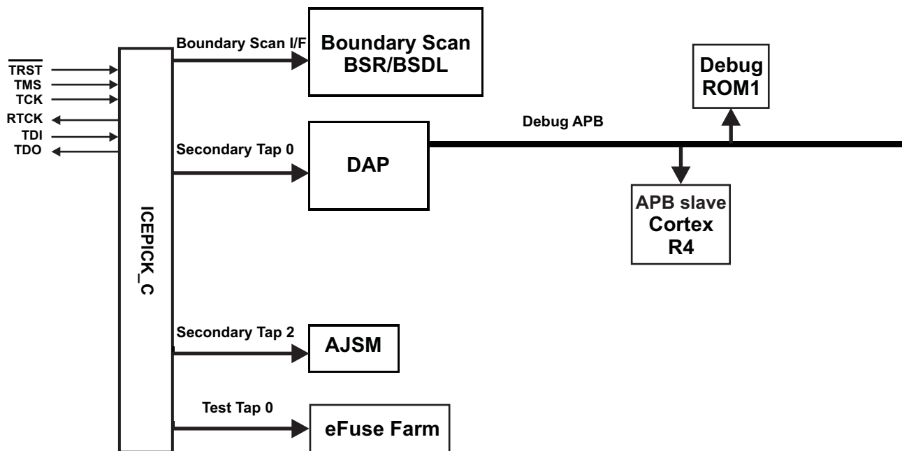
Figure 4-13. ZWT Debug Subsystem Block Diagram
