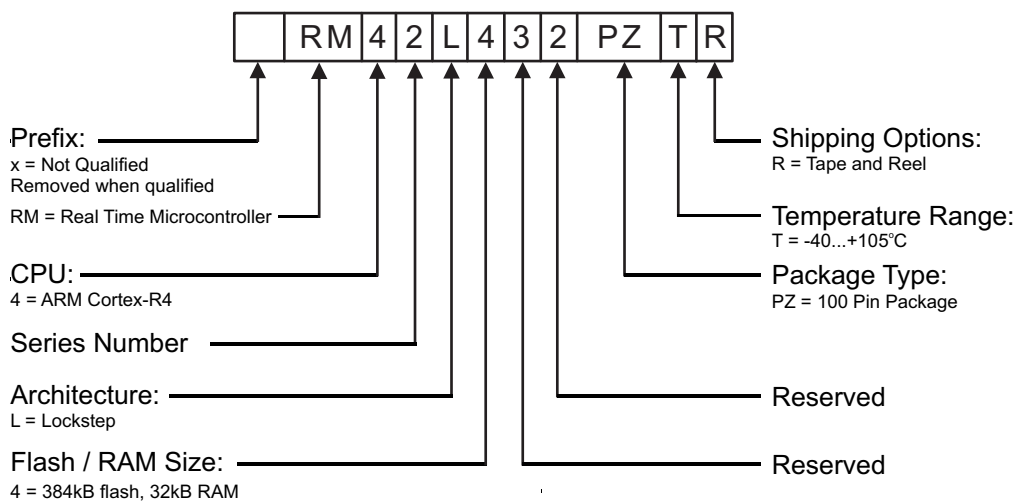
Figure 6-1. Device Numbering Conventions
