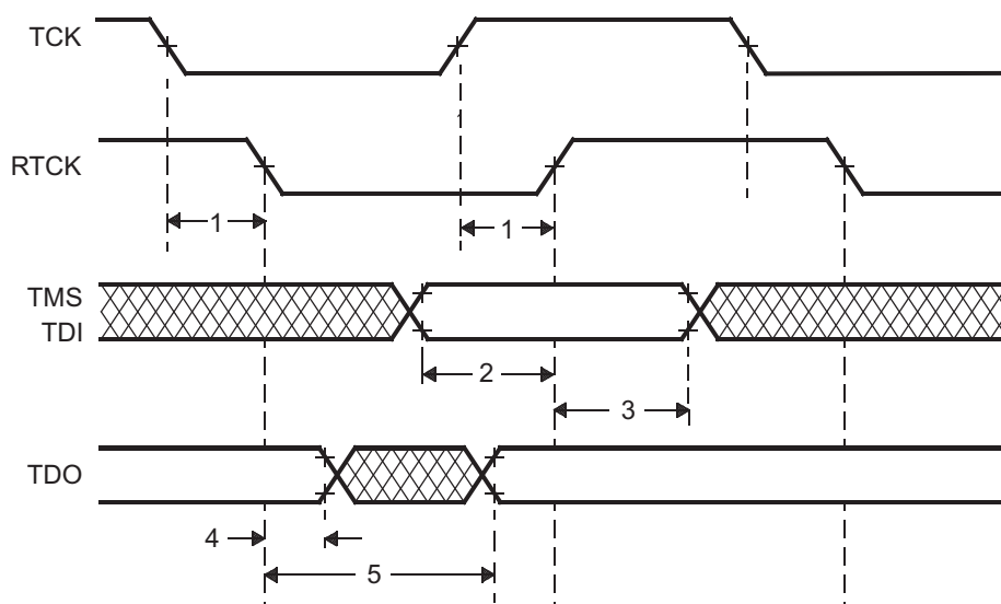
Figure 4-14. JTAG Timing
