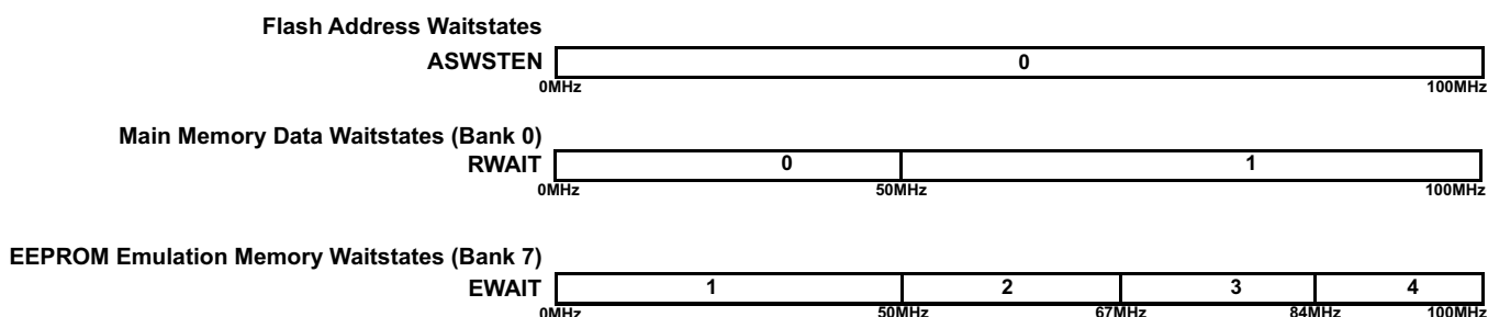
Figure 3-1. Wait States Scheme
