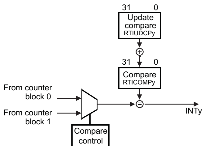
Figure 4-12. Compare Block Diagram
