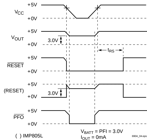
Figure 2. Timing Diagram
