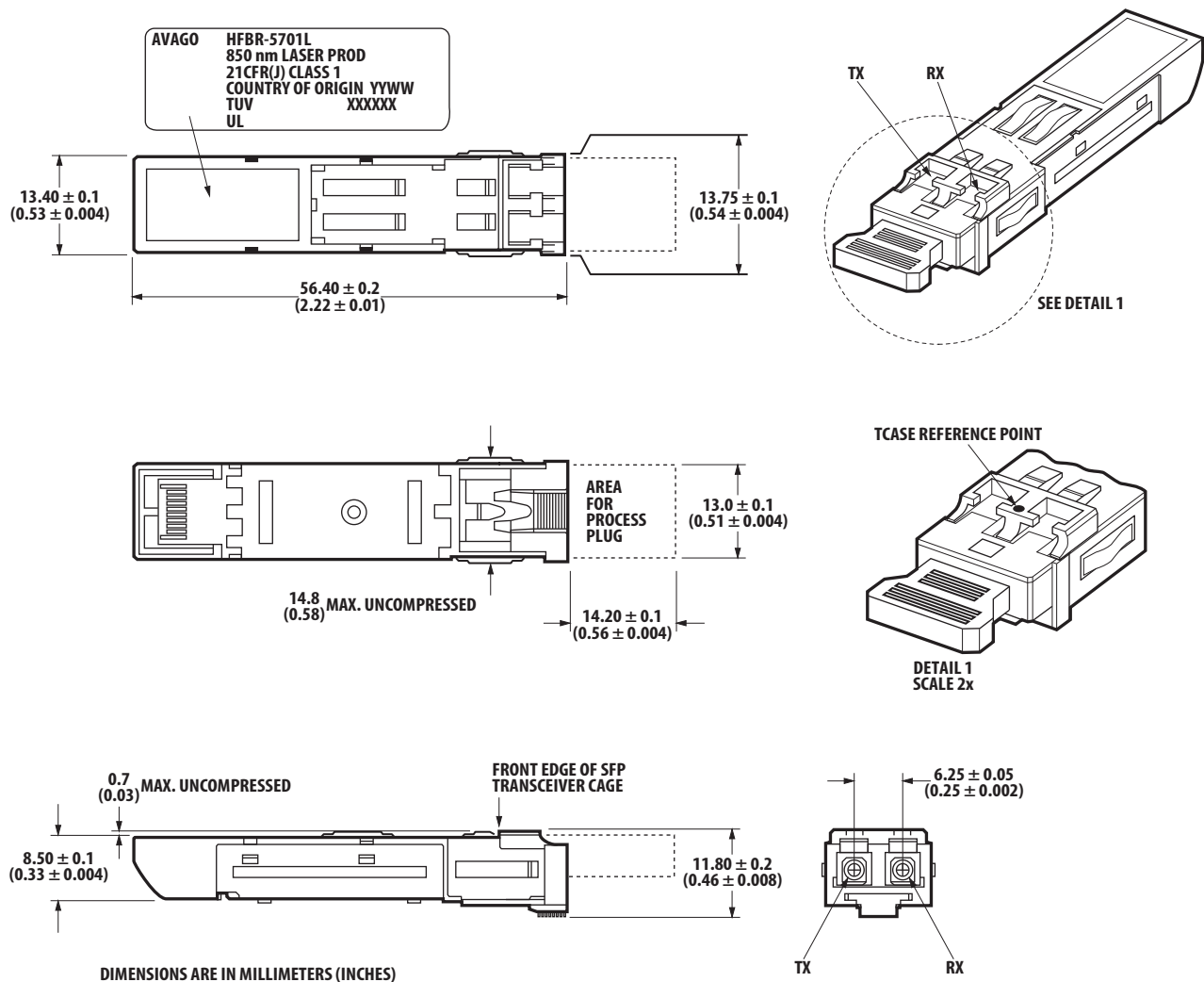
Figure 7. Module drawing.
