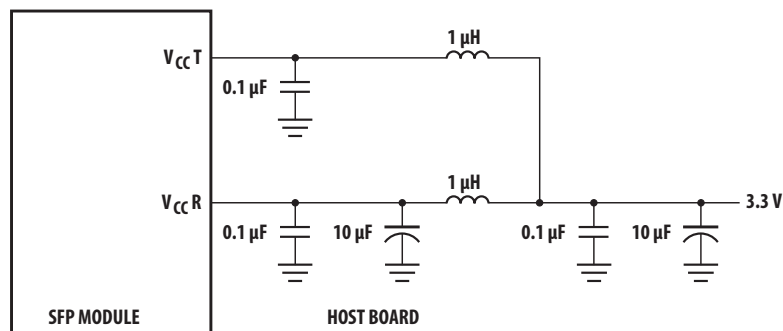
Figure 3. MSA required power supply filter.
